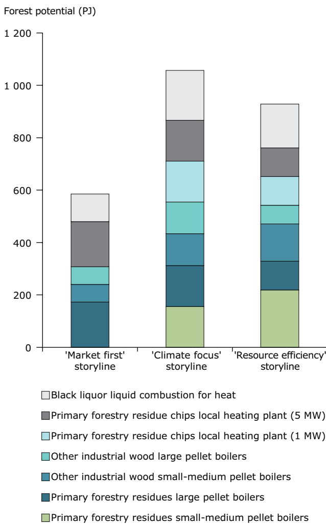
Figure 5.7 Forest potential (PJ) and technology mix per storyline in 2020
